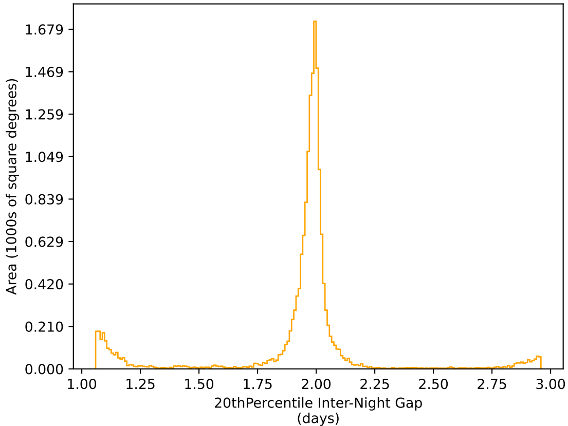
too_ignore_5_4v3.4_10yrs WFD r band: 20thPercentile Inter-Night Gap
