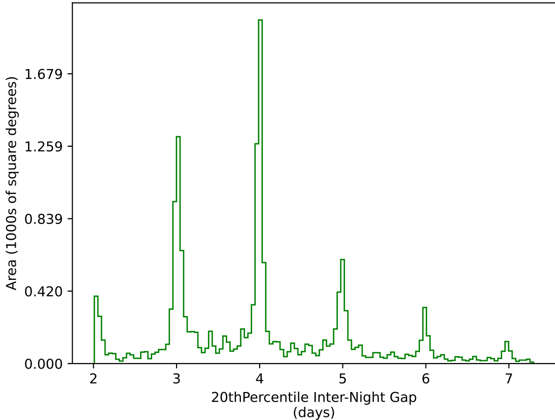
too_ignore_5_4v3.4_10yrs WFD g band: 20thPercentile Inter-Night Gap
