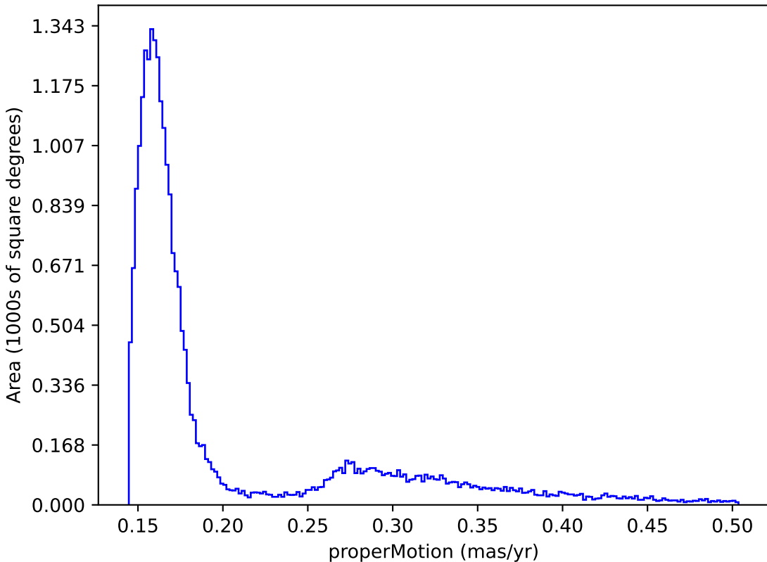
too_ignore_5_4v3.4_10yrs : properMotion
