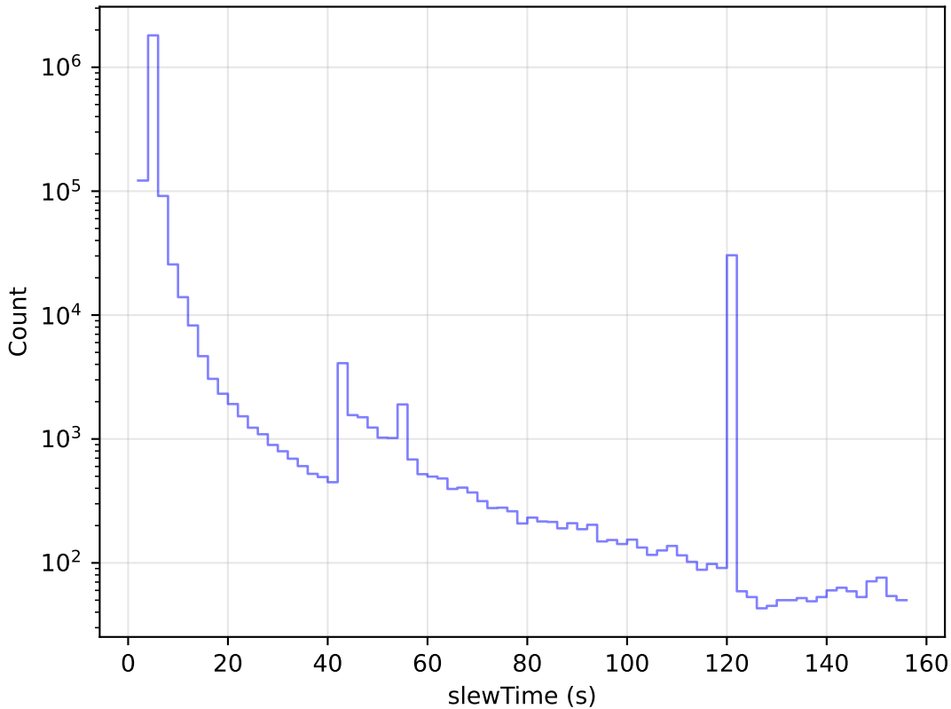
too_ignore_5_4v3.4_10yrs All visits: Slew Time Histogram
