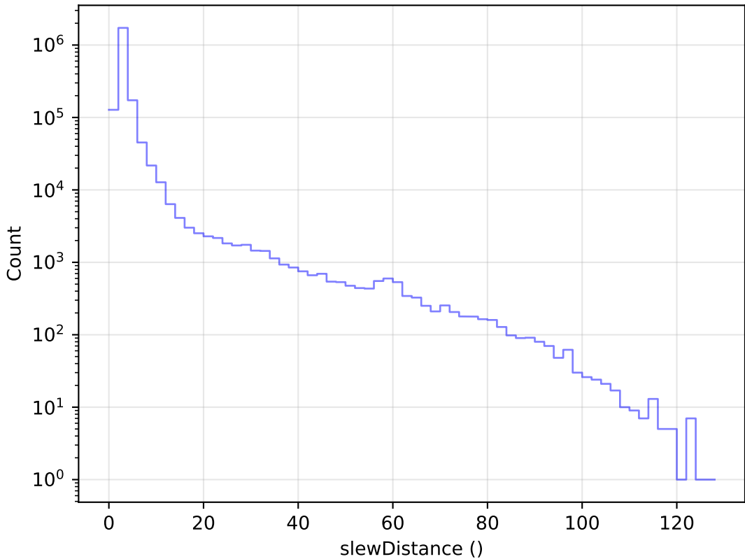
too_ignore_5_4v3.4_10yrs All visits: Slew Distance Histogram
