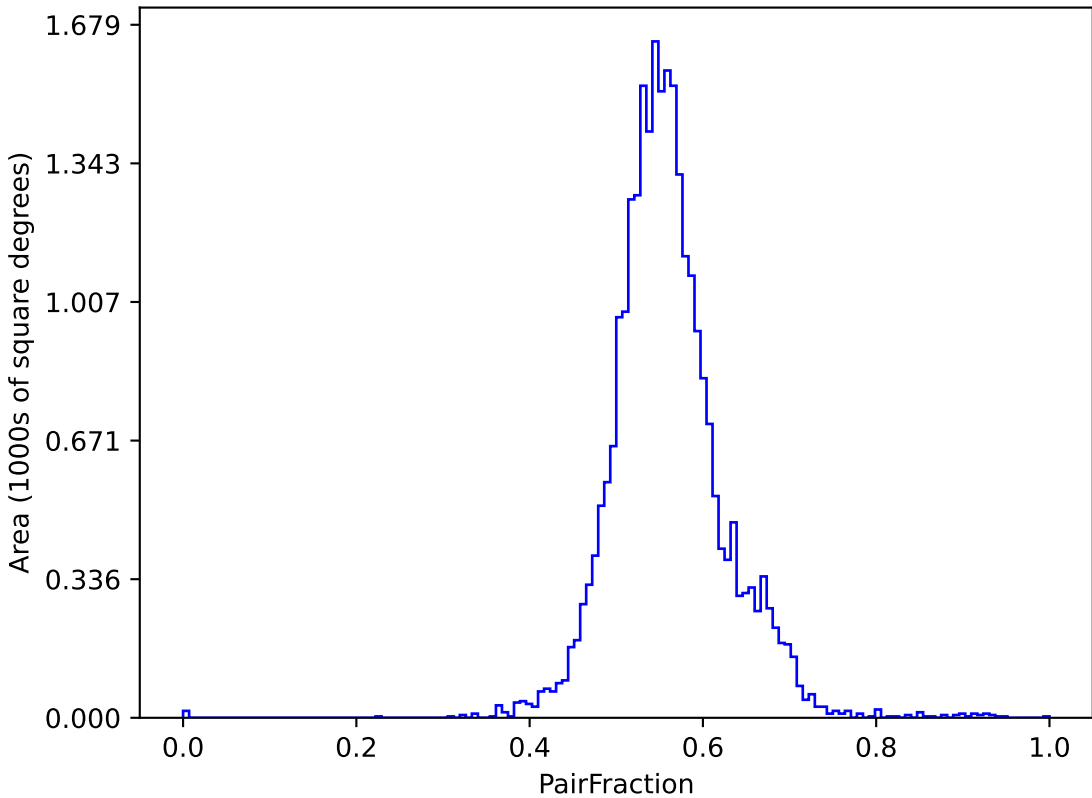
too_ignore_5_4v3.4_10yrs (g or r or i): PairFraction
