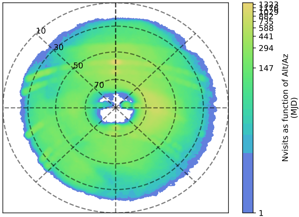
too_ignore_5_4v3.4_10yrs g: Nvisits as function of Alt/Az
