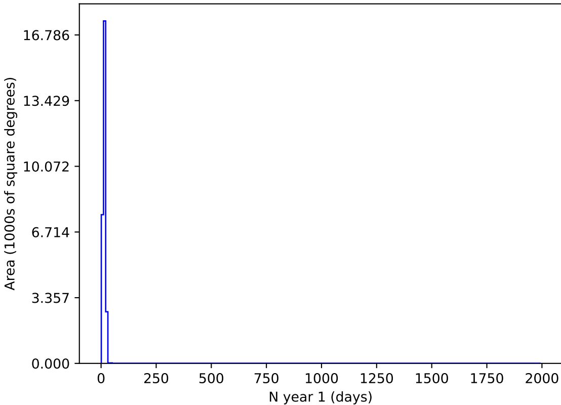
too_ignore_5_4v3.4_10yrs z and night < 365: N year 1
