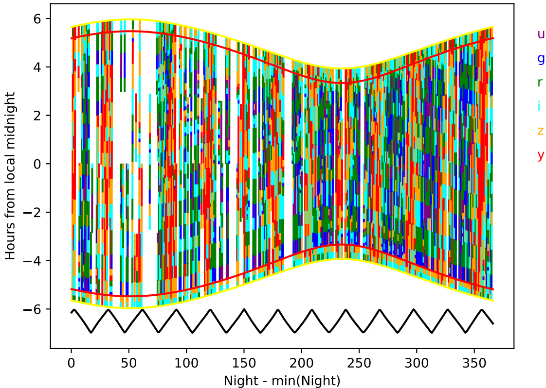
too_ignore_5_4v3.4_10yrs year 9-10: Hourglass
