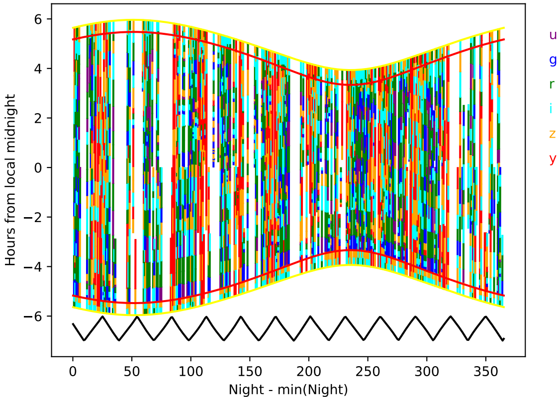
too_ignore_5_4v3.4_10yrs year 7-8: Hourglass
