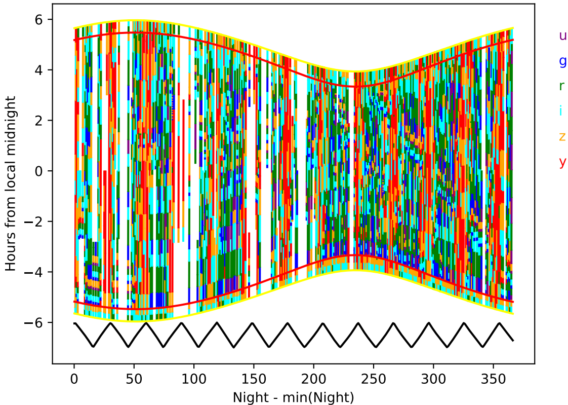
too_ignore_5_4v3.4_10yrs year 1-2: Hourglass
