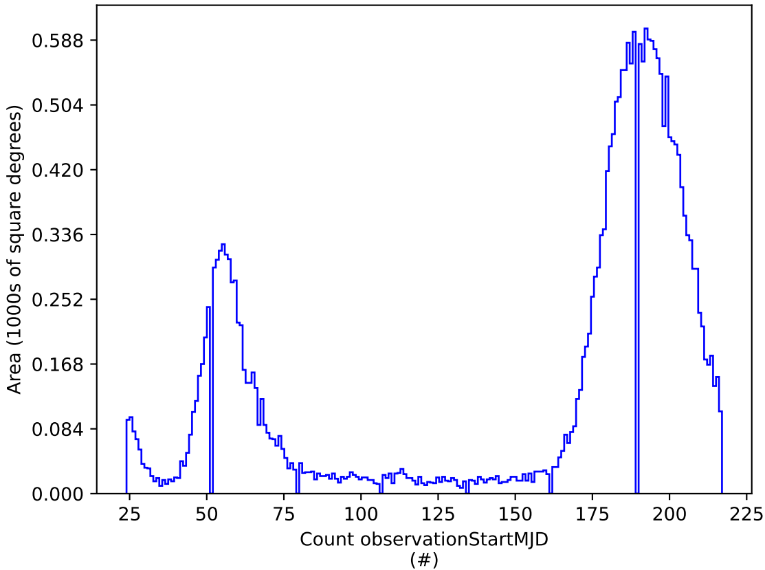
too_ignore_5_4v3.4_10yrs i: Count observationStartMJD
