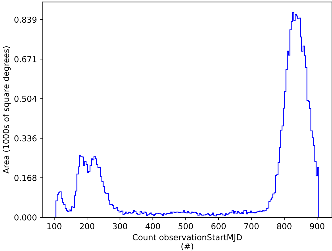
too_ignore_5_4v3.4_10yrs : Count observationStartMJD
