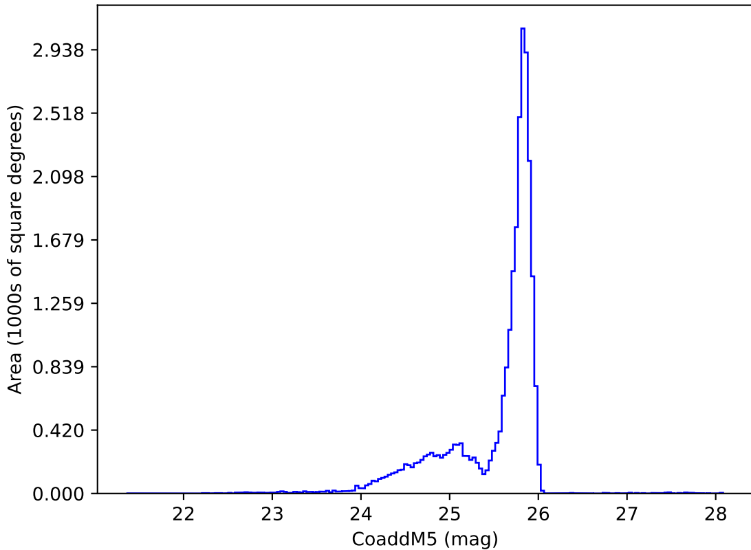
too_ignore_5_4v3.4_10yrs z: CoaddM5
