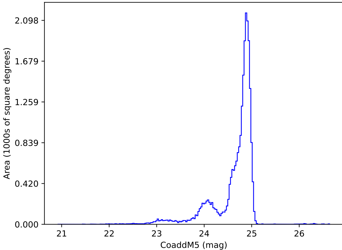
too_ignore_5_4v3.4_10yrs y: CoaddM5
