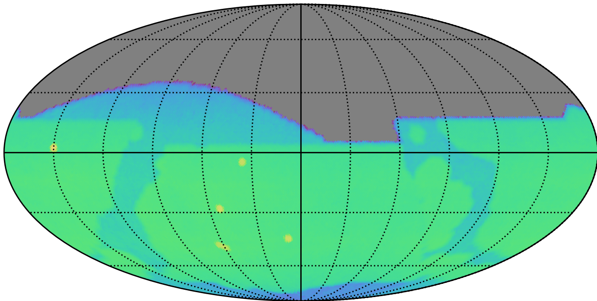
too_ignore_5_4v3.4_10yrs r: CoaddM5
