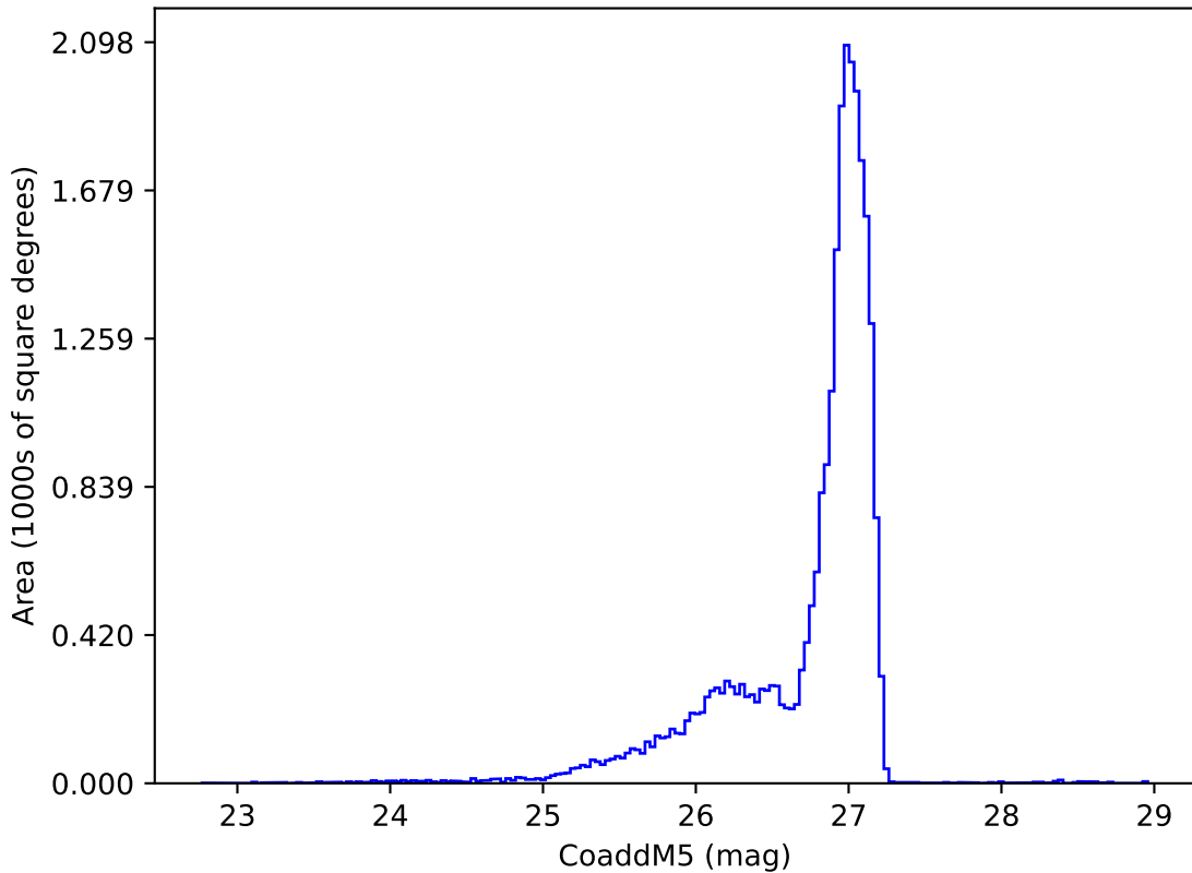
too_ignore_5_4v3.4_10yrs r: CoaddM5
