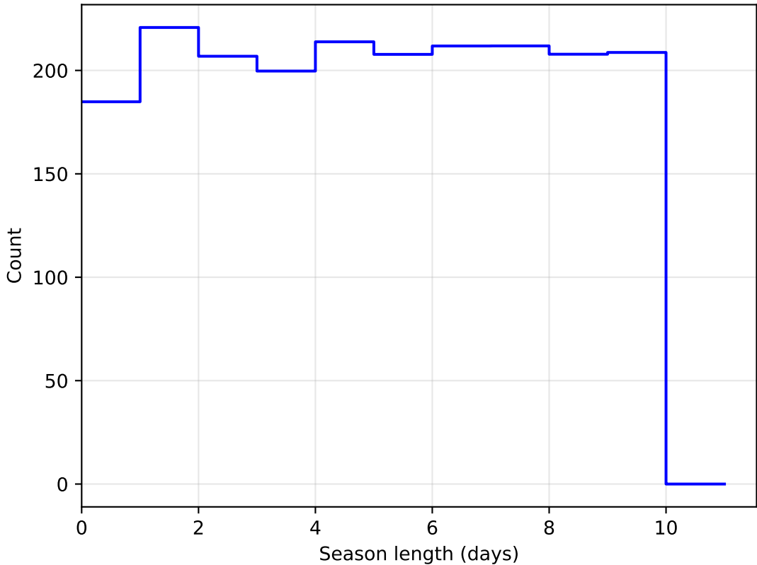
too_ignore_5_4v3.4_10yrs DD:ELAISS1 all bands: SeasonLength
