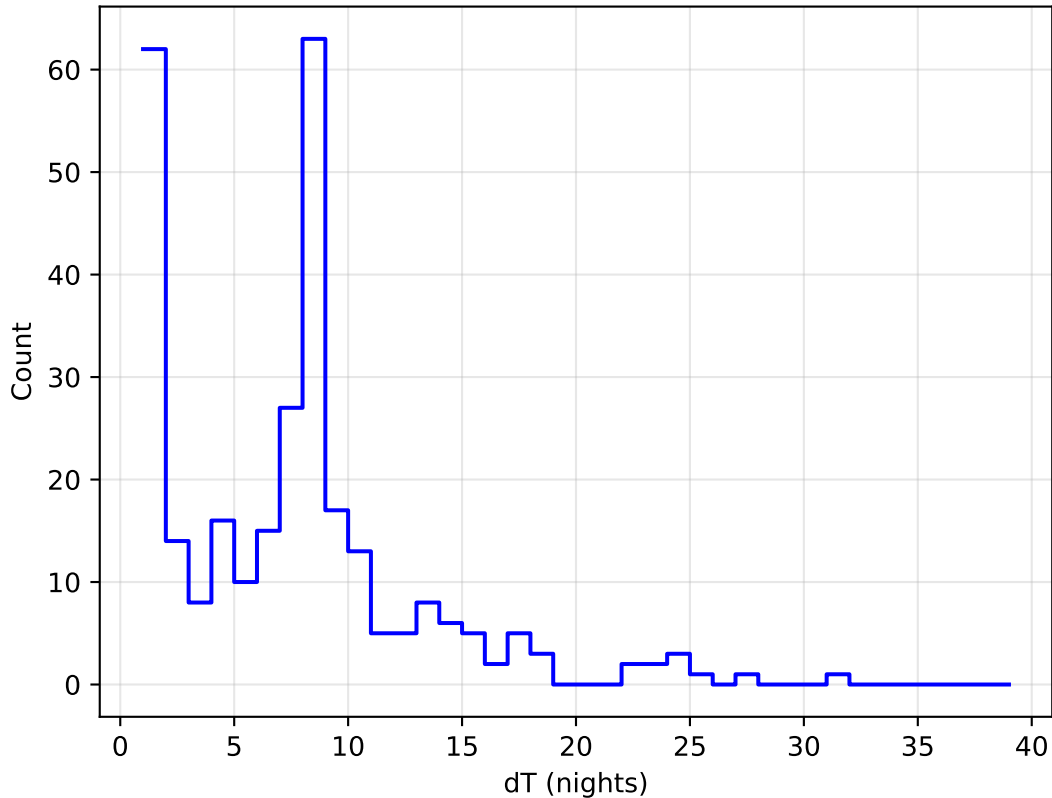
too_ignore_5_4v3.4_10yrs all bands: DD:XMM_LSS Delta Nights Histogram
