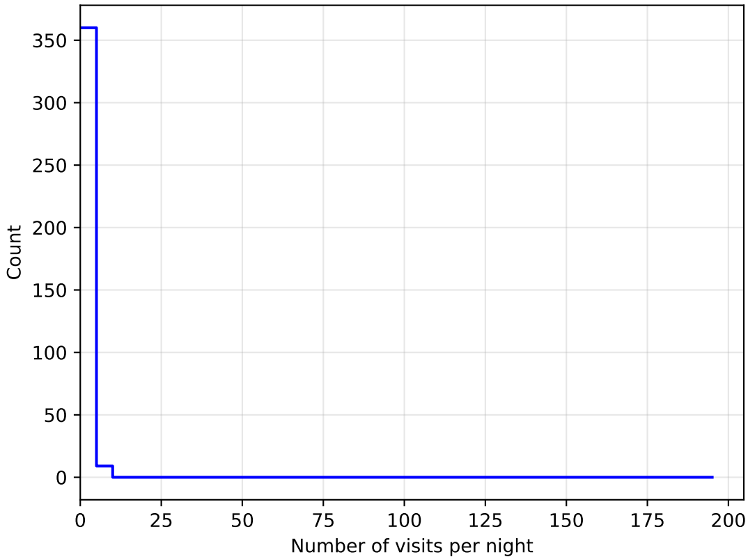
too_ignore_5_4v3.4_10yrs all bands: DD:WFD NVisitsPerNight
