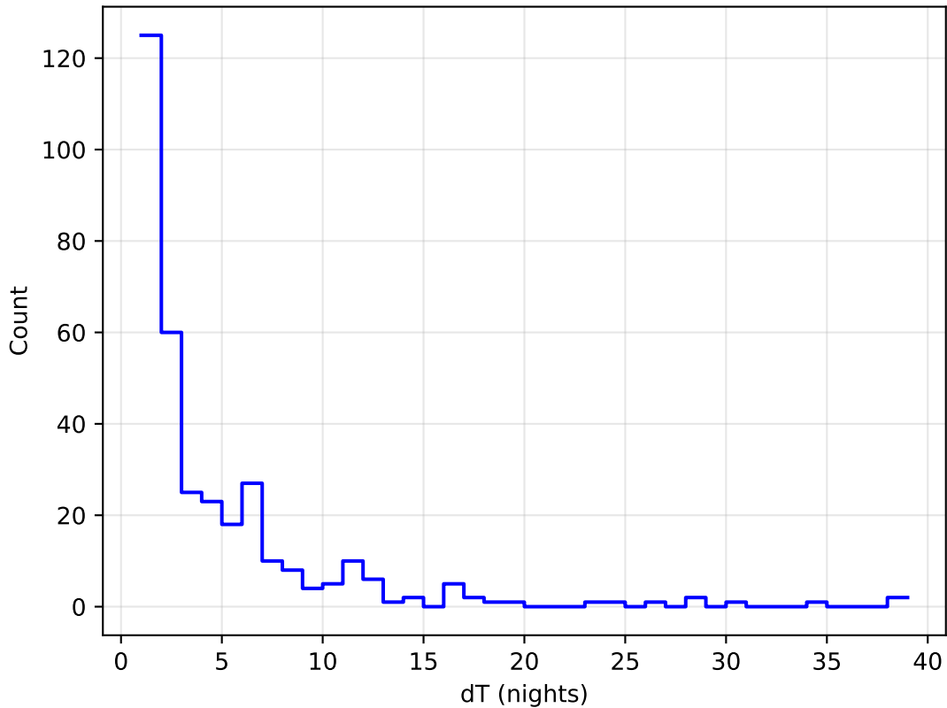
too_ignore_5_4v3.4_10yrs all bands: DD:WFD Delta Nights Histogram
