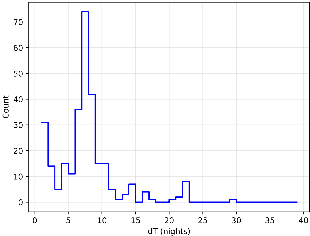
too_ignore_5_4v3.4_10yrs all bands: DD:EDFS Delta Nights Histogram
