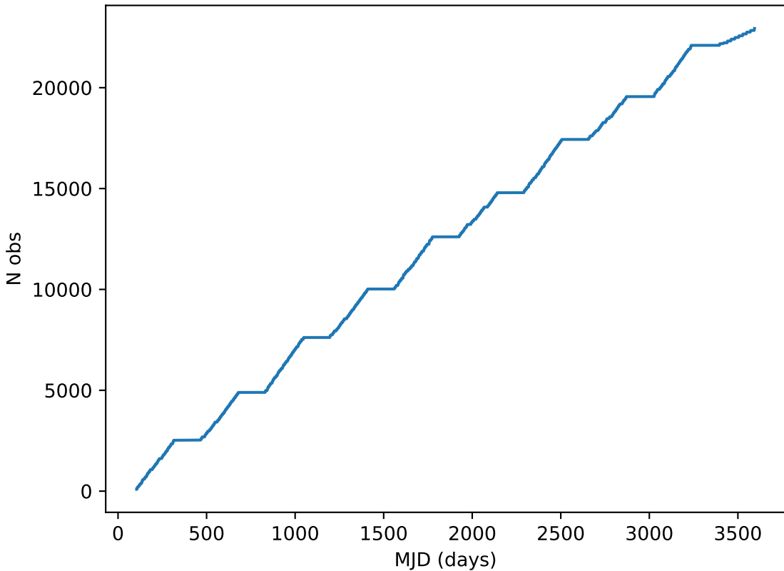
too_ignore_5_4v3.4_10yrs all bands: DD:EDFS Cumulative NVisits
