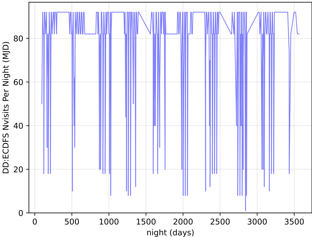
too_ignore_5_4v3.4_10yrs all bands: DD:ECDFS Nvisits Per Night
