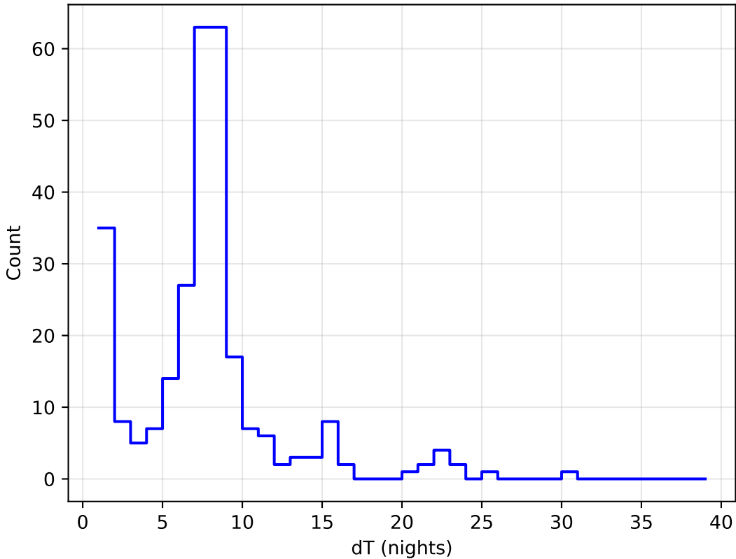
too_ignore_5_4v3.4_10yrs all bands: DD:ECDFS Delta Nights Histogram
