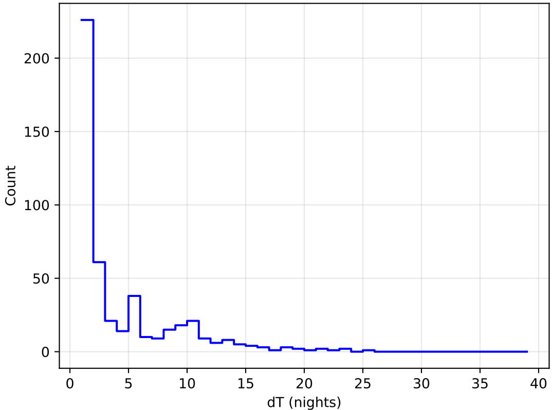
too_ignore_5_4v3.4_10yrs all bands: DD: COSMOS Delta Nights Histogram
