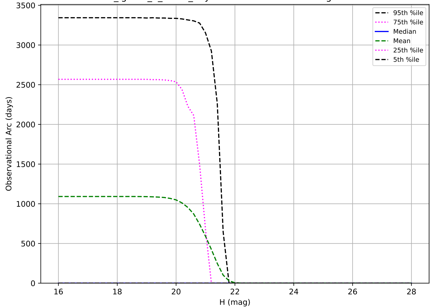
too_ignore_5_1v3.4_10yrs: Observational Arc Length Vatira
