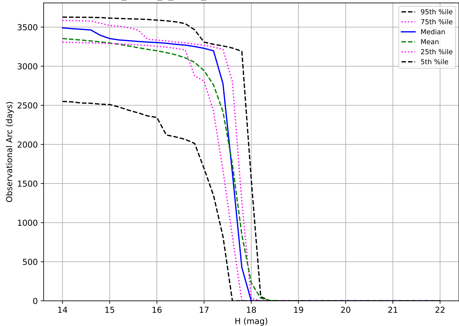
too_ignore_5_1v3.4_10yrs: Observational Arc Length Trojan
