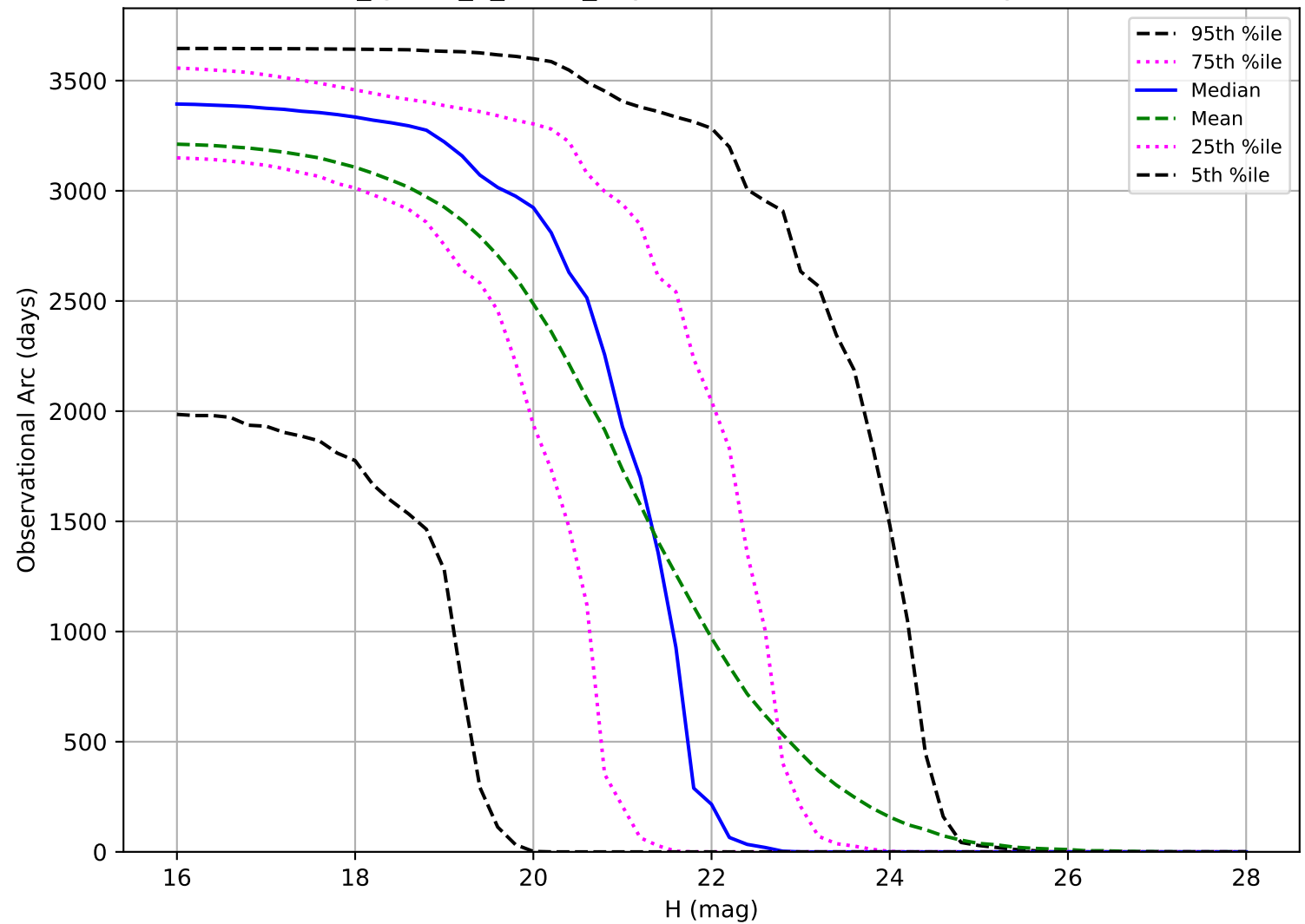
too_ignore_5_1v3.4_10yrs: Observational Arc Length PHA
