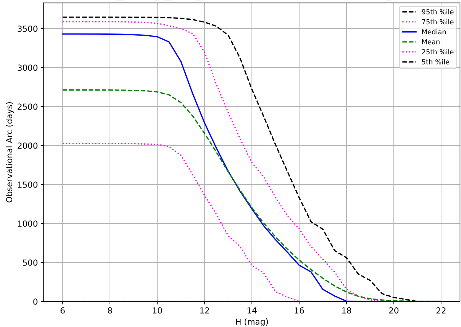
too_ignore_5_1v3.4_10yrs: Observational Arc Length OCC_r5
