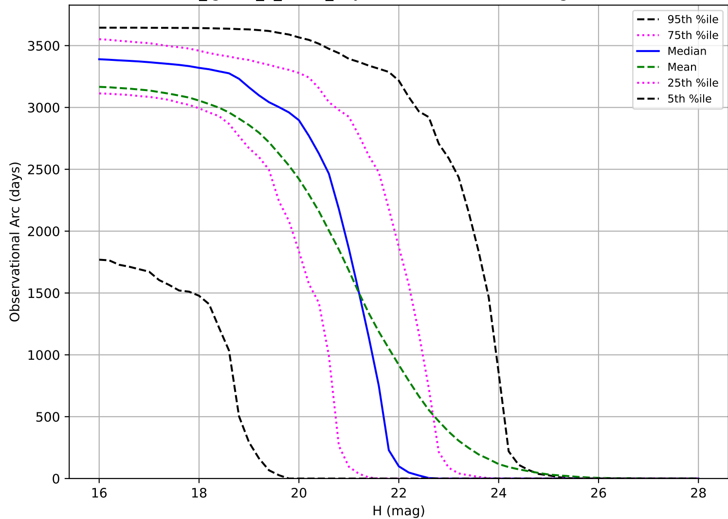
too_ignore_5_1v3.4_10yrs: Observational Arc Length NEO
