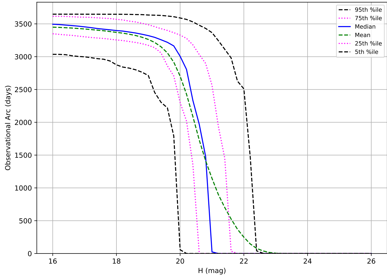
too_ignore_5_1v3.4_10yrs: Observational Arc Length MBA
