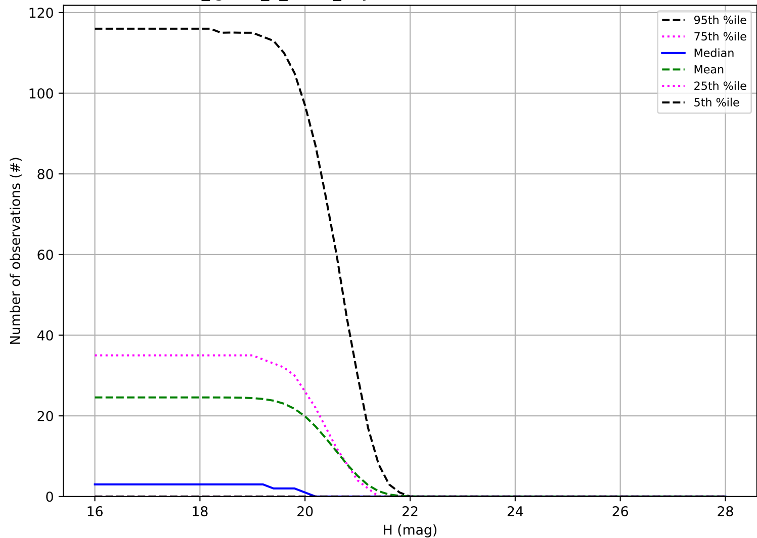
too_ignore_5_1v3.4_10yrs: Number of observations Vatira
