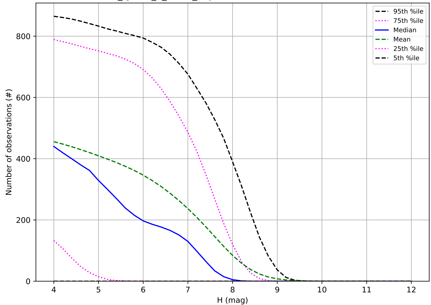
too_ignore_5_1v3.4_10yrs: Number of observations TNO
