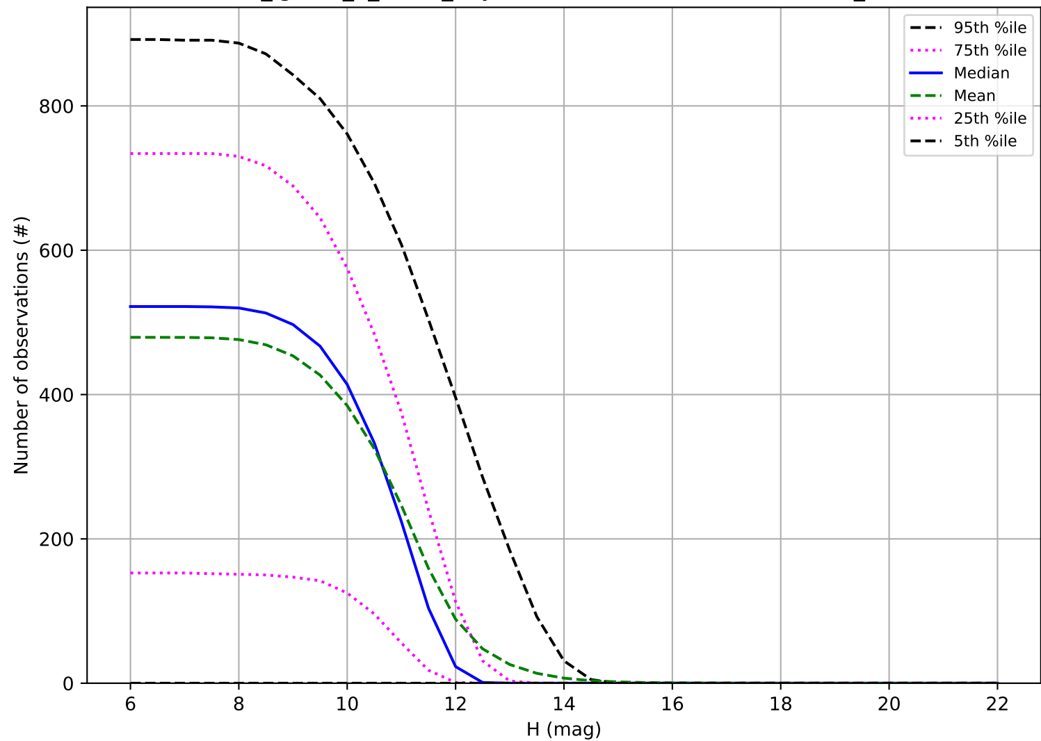
too_ignore_5_1v3.4_10yrs: Number of observations OCC_r20
