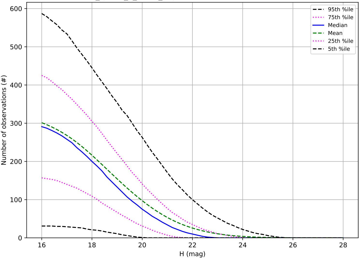
too_ignore_5_1v3.4_10yrs: Number of observations NEO
