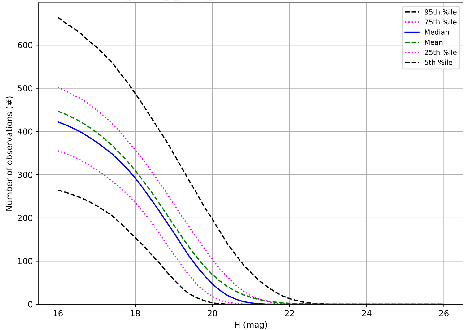
too_ignore_5_1v3.4_10yrs: Number of observations MBA
