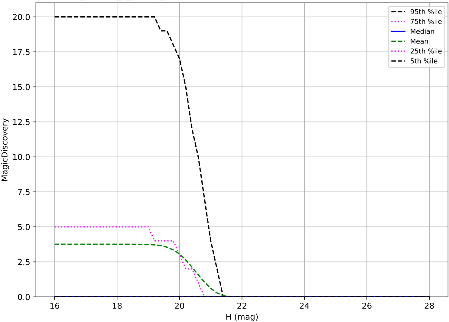
too_ignore_5_1v3.4_10yrs: Vatira 6 detections in 60 nights detection loss
