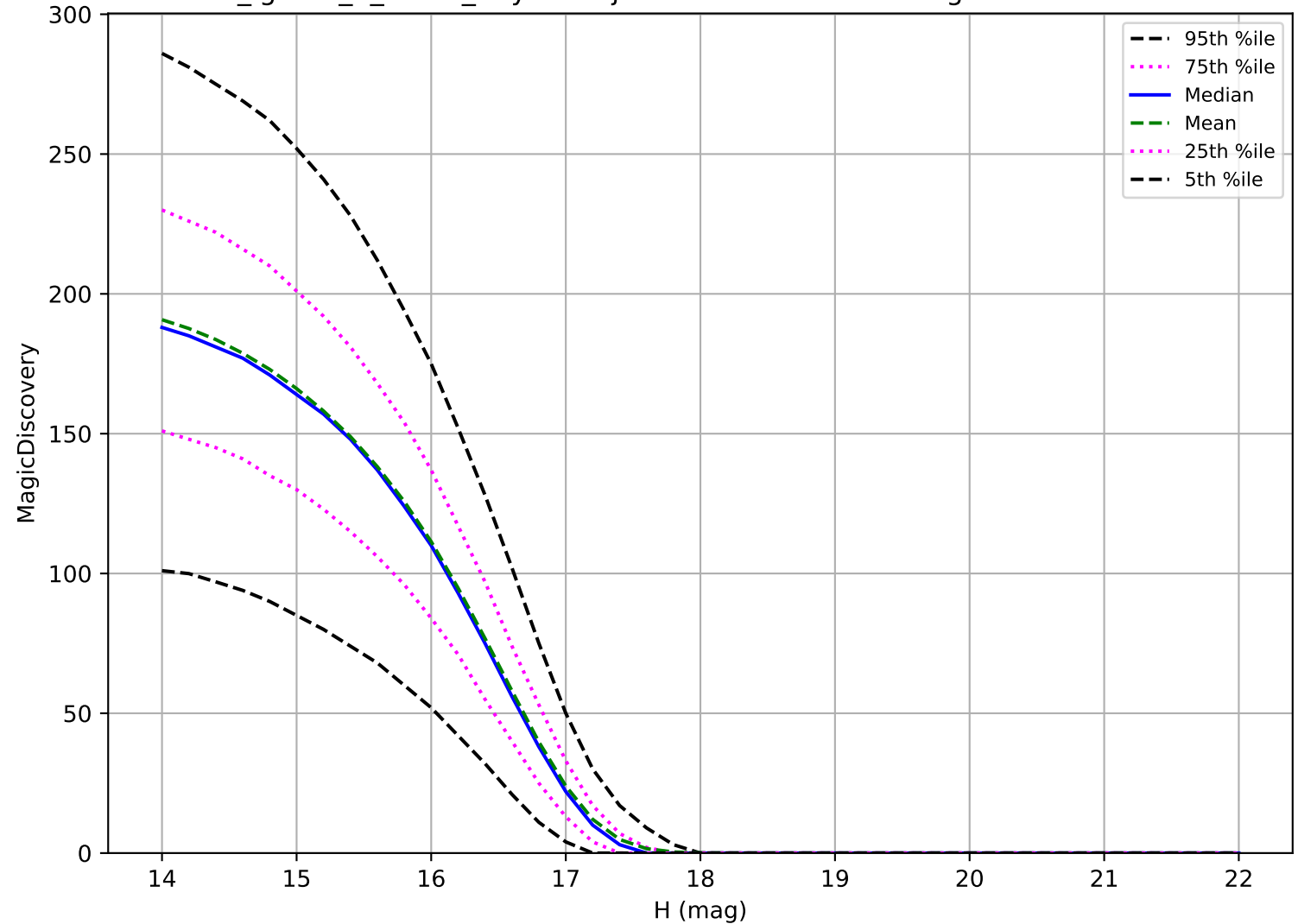
too_ignore_5_1v3.4_10yrs: Trojan 6 detections in 60 nights detection loss
