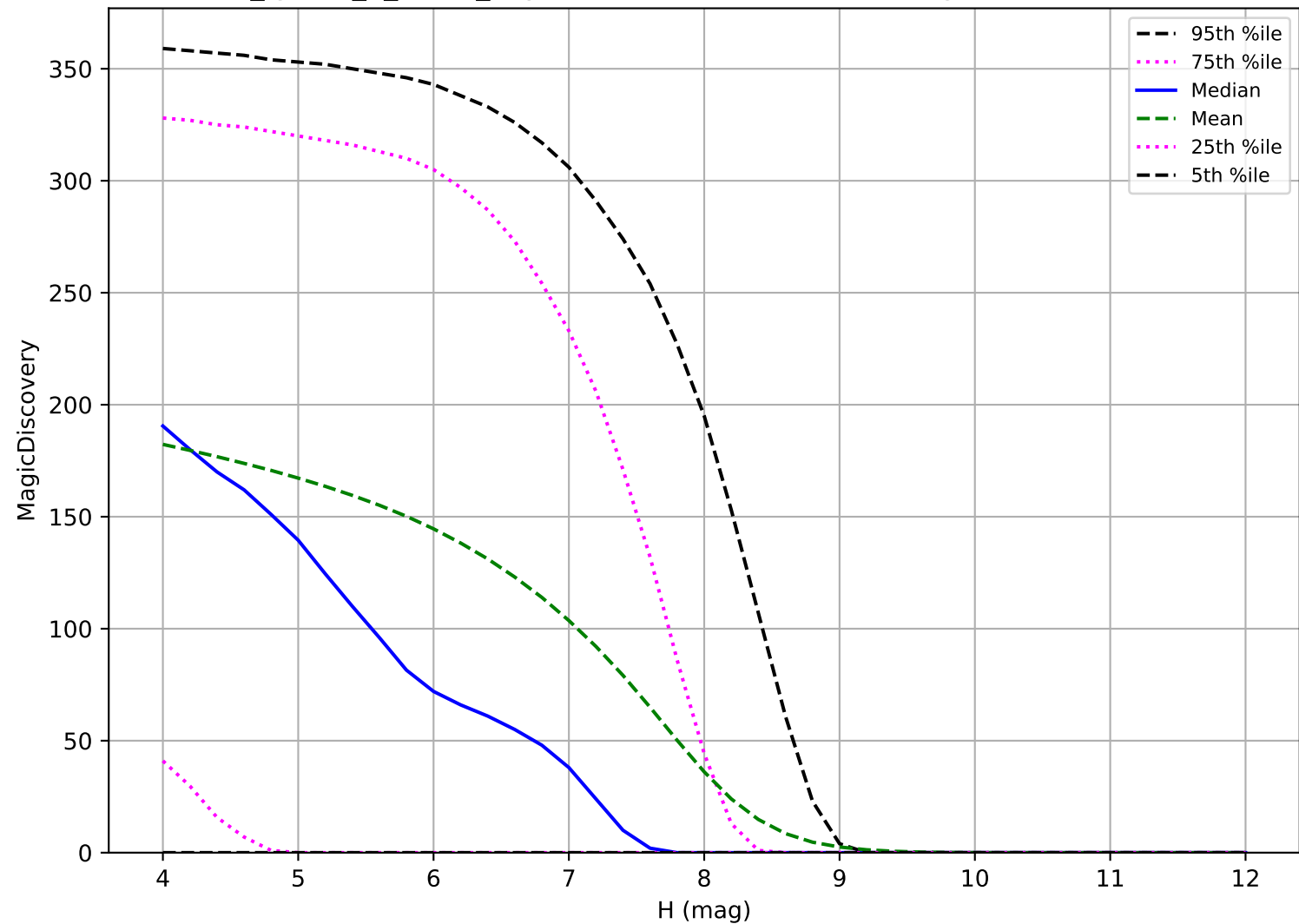
too_ignore_5_1v3.4_10yrs: TNO 6 detections in 60 nights detection loss
