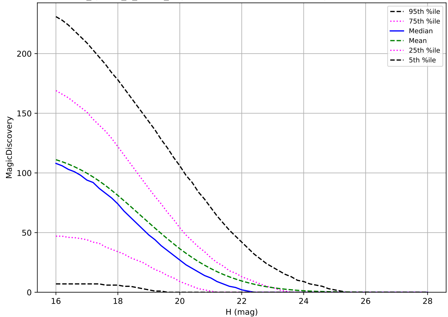
too_ignore_5_1v3.4_10yrs: PHA 6 detections in 60 nights detection loss
