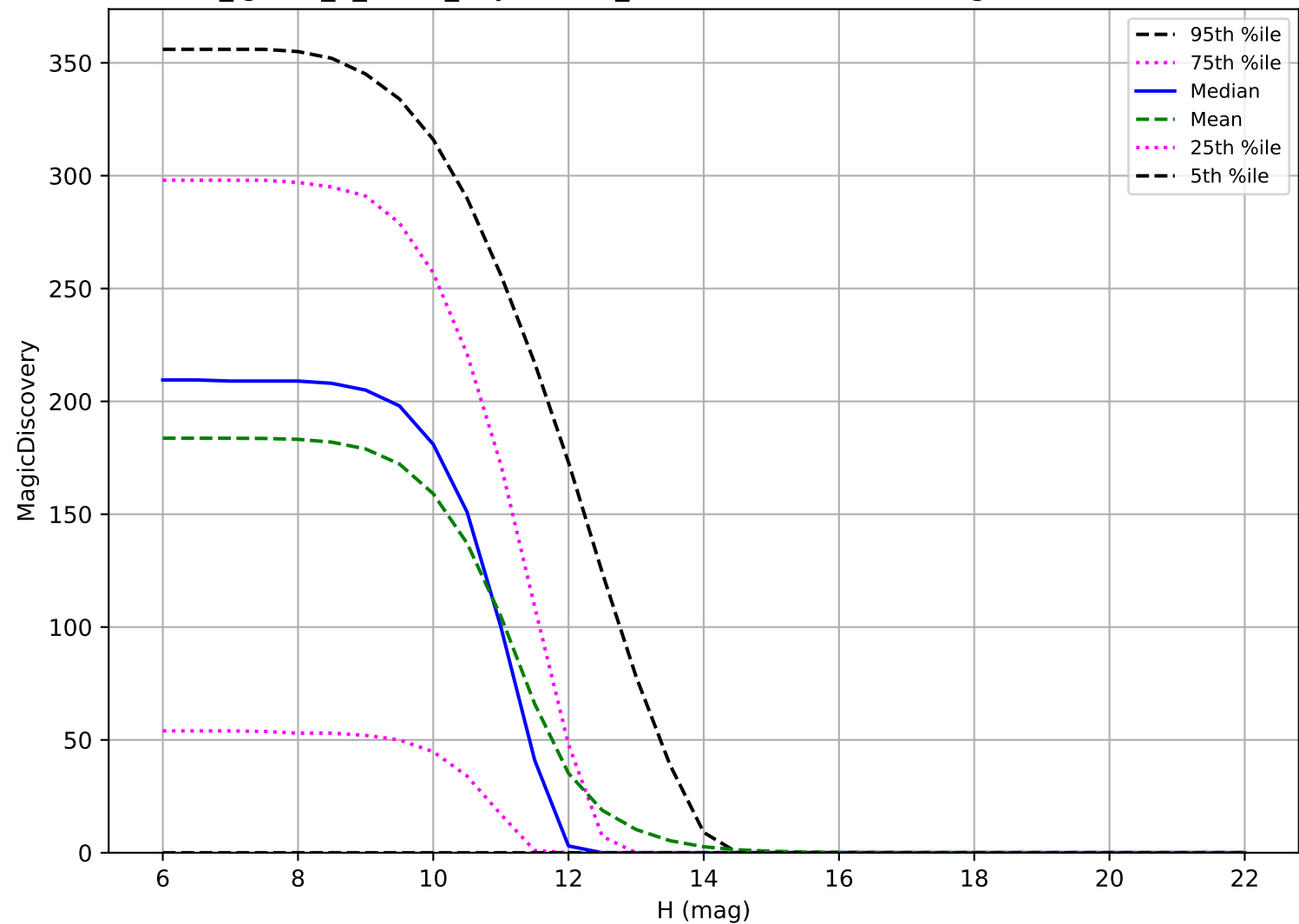
too_ignore_5_1v3.4_10yrs: OCC_r20 6 detections in 60 nights detection loss
