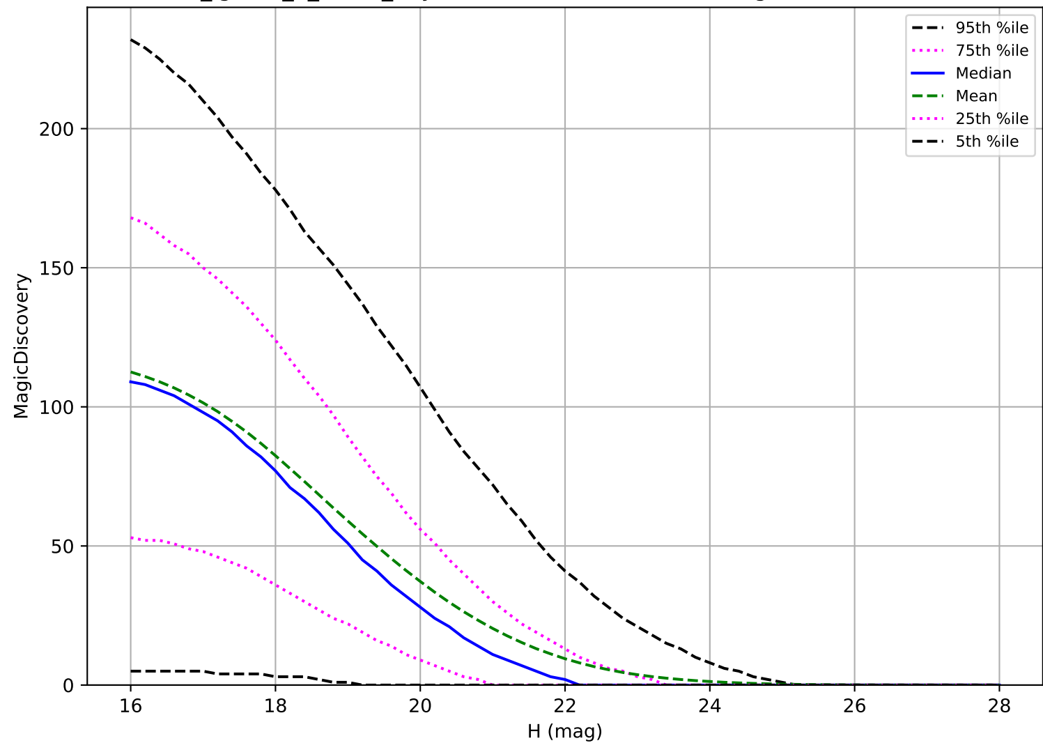
too_ignore_5_1v3.4_10yrs: NEO 6 detections in 60 nights detection loss
