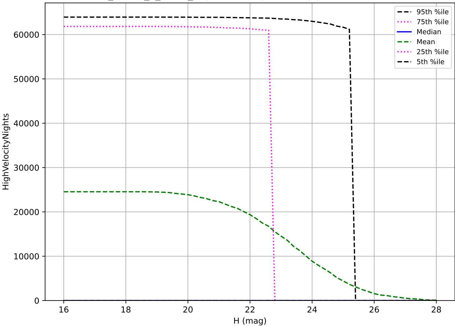
too_ignore_5_1v3.4_10yrs: PHA High velocity pair detection loss
