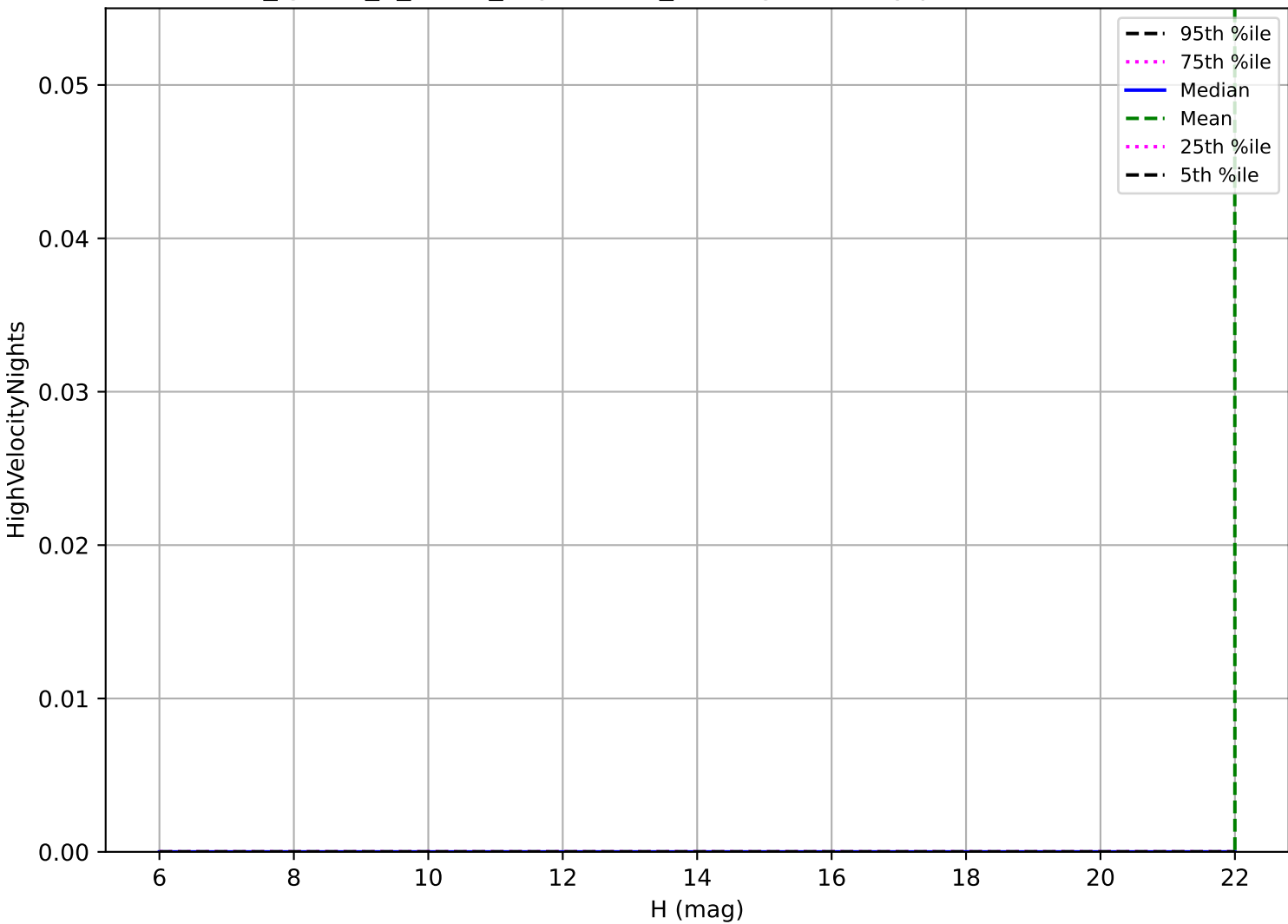
too_ignore_5_1v3.4_10yrs: OCC_r20 High velocity pair detection loss
