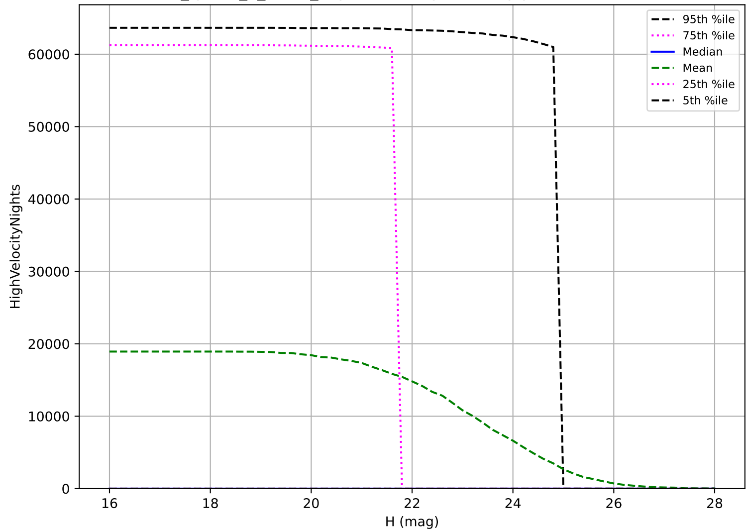
too_ignore_5_1v3.4_10yrs: NEO High velocity pair detection loss
