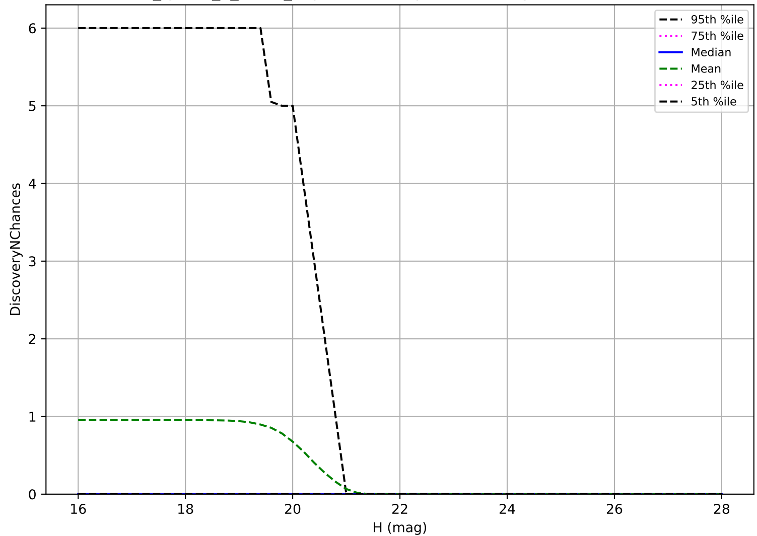
too_ignore_5_1v3.4_10yrs: Vatira 3 pairs in 15 nights detection loss
