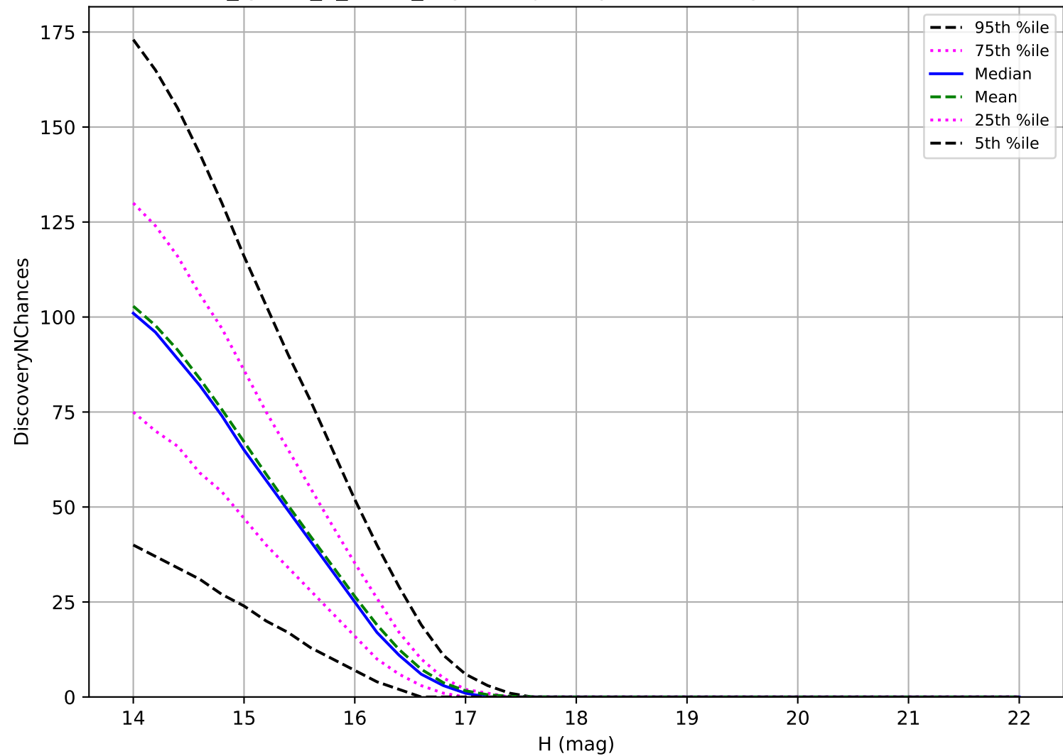
too_ignore_5_1v3.4_10yrs: Trojan 3 pairs in 15 nights detection loss
