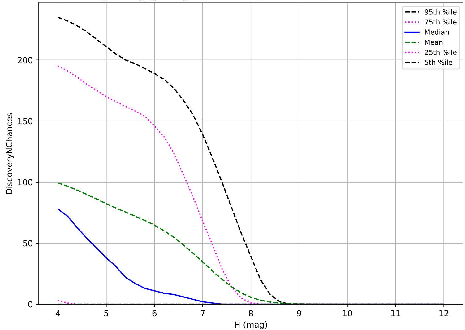
too_ignore_5_1v3.4_10yrs: TNO 3 pairs in 15 nights detection loss
