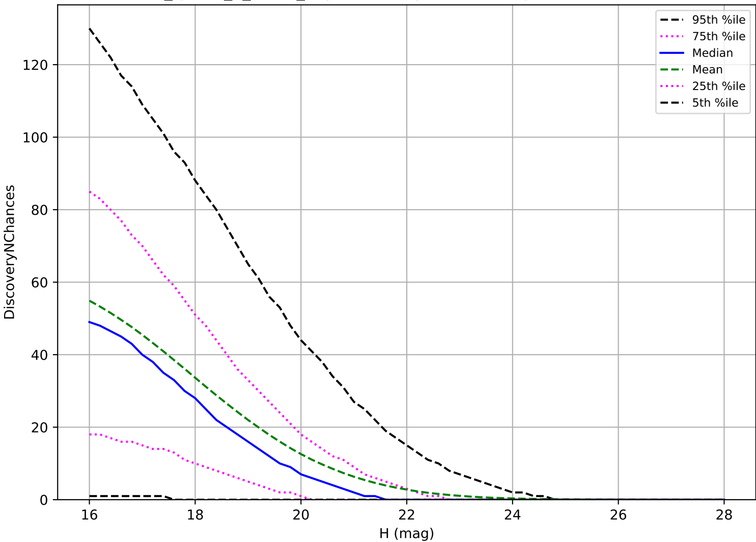
too_ignore_5_1v3.4_10yrs: PHA 3 pairs in 15 nights detection loss
